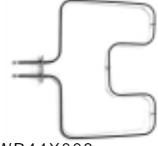
WB44X228 G.E. Bake Element, fixed, 18-1/4" X 15-1/2", 3000W, 240V.
