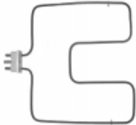
WB44X5019 G.E. Bake Element, fixed/ ceramic, 15-1/2" X 15", 3000W, 240V.
