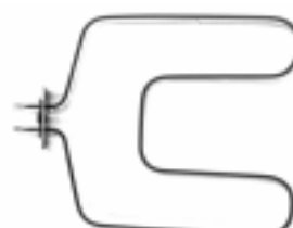
WB44X190 G.E. Bake Element, hinged, 13-1/2" X 16", 2585W, 240V.
