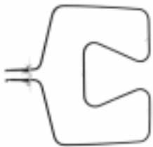
WB44X164 G.E. Bake Element, hinged, 18" X 15-3/4", 3000W, 240V.
