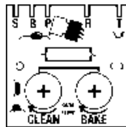
WB24X162 G.E./Hotpoint Terminal Board For Self Cleaning Oven.
